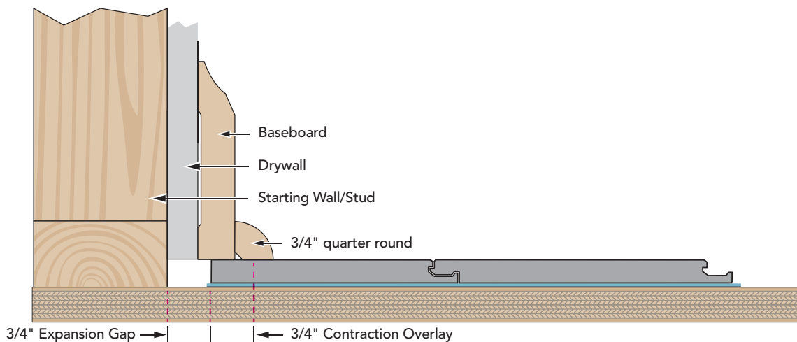
TYPICAL INSTALLATION
