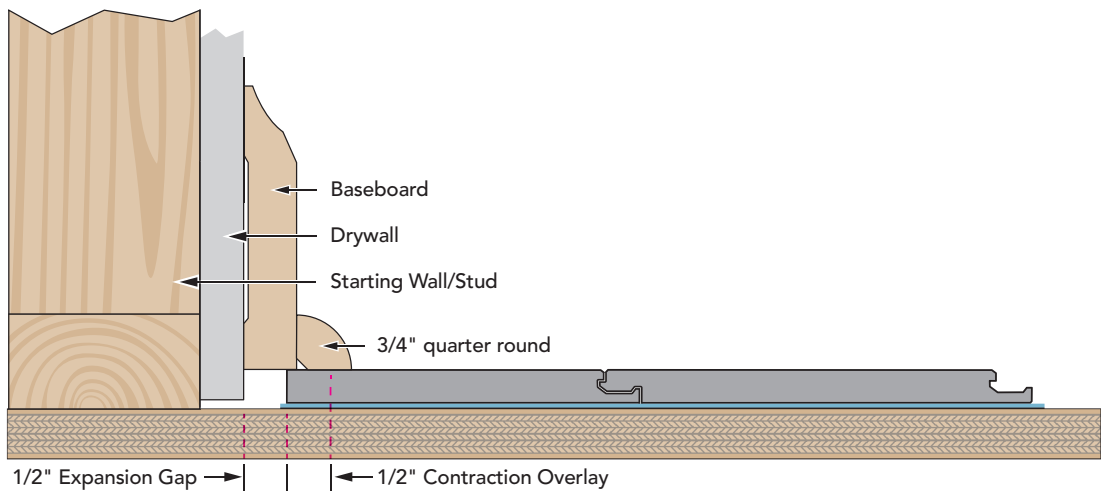
TYPICAL INSTALLATION
