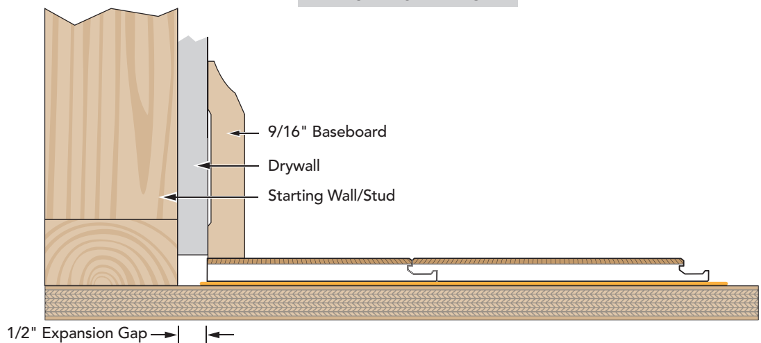
How to achieve required Expansion Gap using base board only
