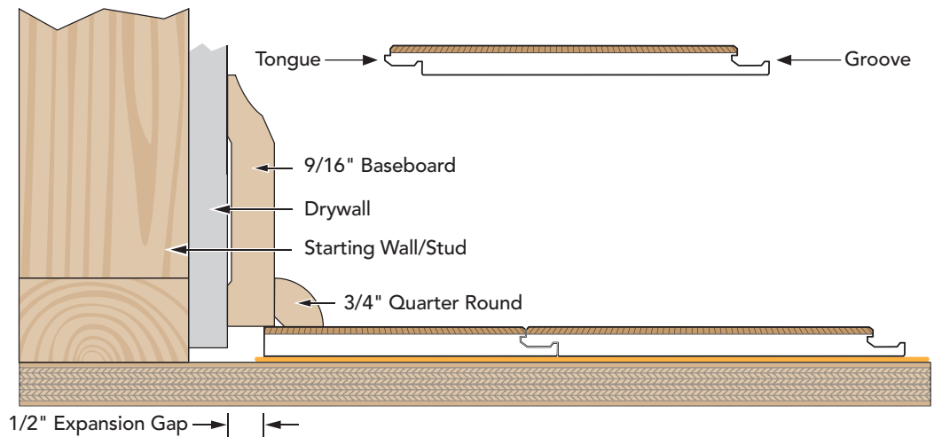
TYPICAL INSTALLATION
