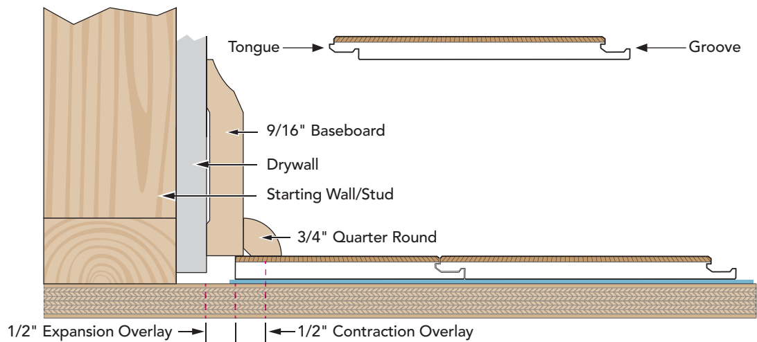
TYPICAL INSTALLATION
